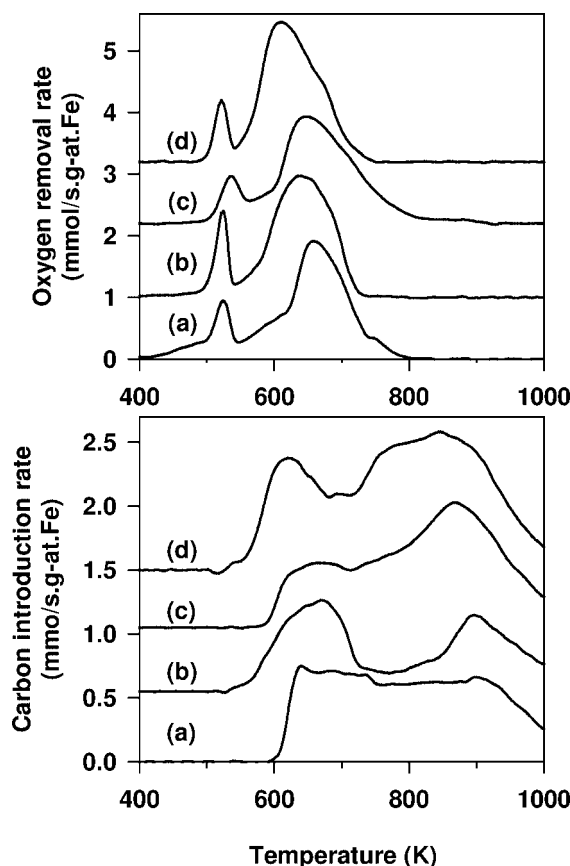
Figure 6. Oxygen removal and carbon introduction rates for the Fe 2 O 3 –Zn–K–Cu (Zn/Fe = 0.1) samples in CO: (a) Fe 2 O 3 –Zn, (b) Fe 2 O 3 –Zn–Cu 1 , (c) Fe 2 O 3 –Zn–K 2 , (d) Fe 2 O 3 –Zn–K 2 –Cu 1 (0.2 g sample, 0.167 K/s ramping rate, 20% CO/Ar, 0.268 mol/h flow rate).
